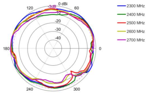
Azimuth: 2300 – 2700 MHz
