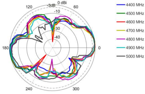
Elevation: 4400 – 5000 MHz
