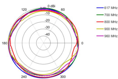
Azimuth: 617 – 960 MHz
