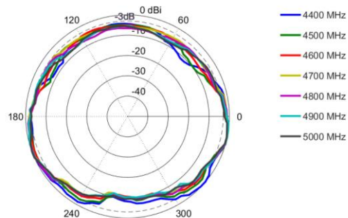
Azimuth: 4400 – 5000 MHz
