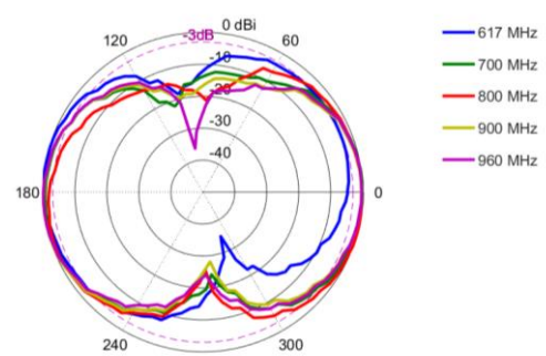
Elevation: 617 – 960 MHz
