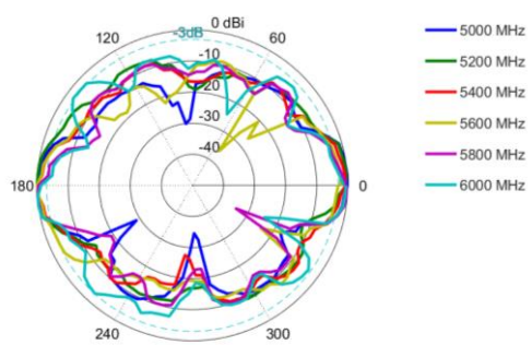
Elevation: 5000 – 6000 MHz
