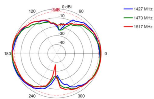
Elevation: 1427 – 1517 MHz
