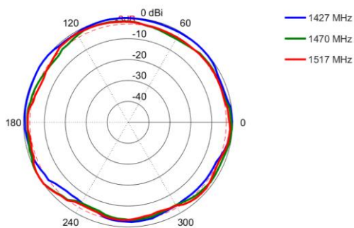
Azimuth: 1427 – 1517 MHz
