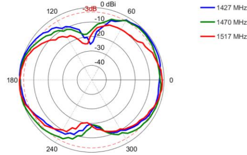
Elevation: 1427 – 1517 MHz
