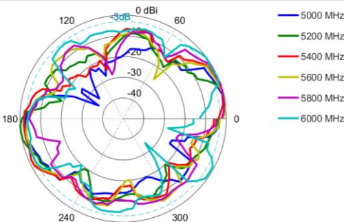
Elevation: 5000 – 6000 MHz
