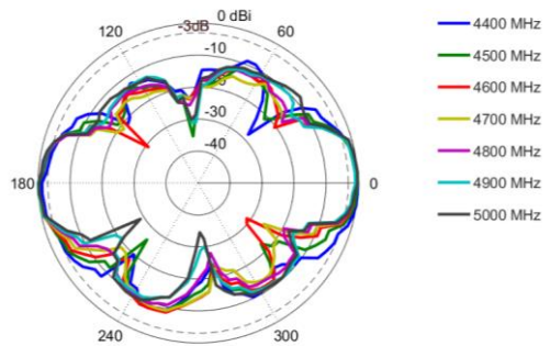
Elevation: 4400 – 5000 MHz
